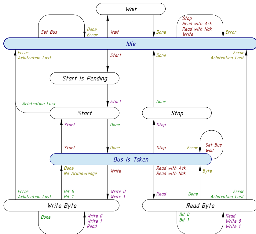
Figure 3: Byte-level FSM
