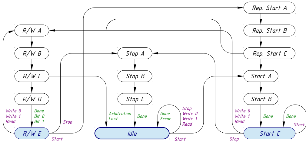
Figure 5: Bit-level FSM
