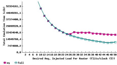
(e) Emulation time in clock cycles.
