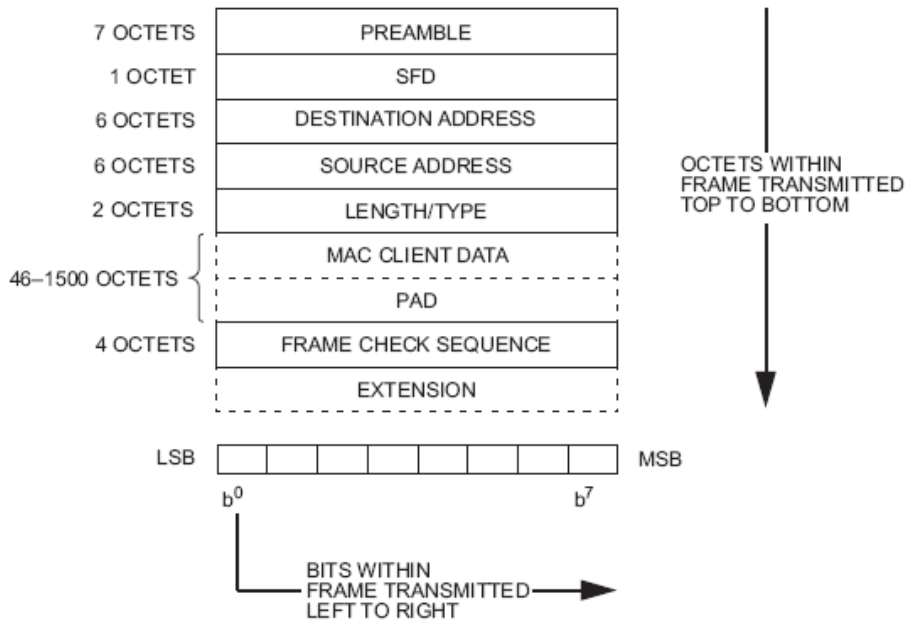
Figure 1 MAC frame format
