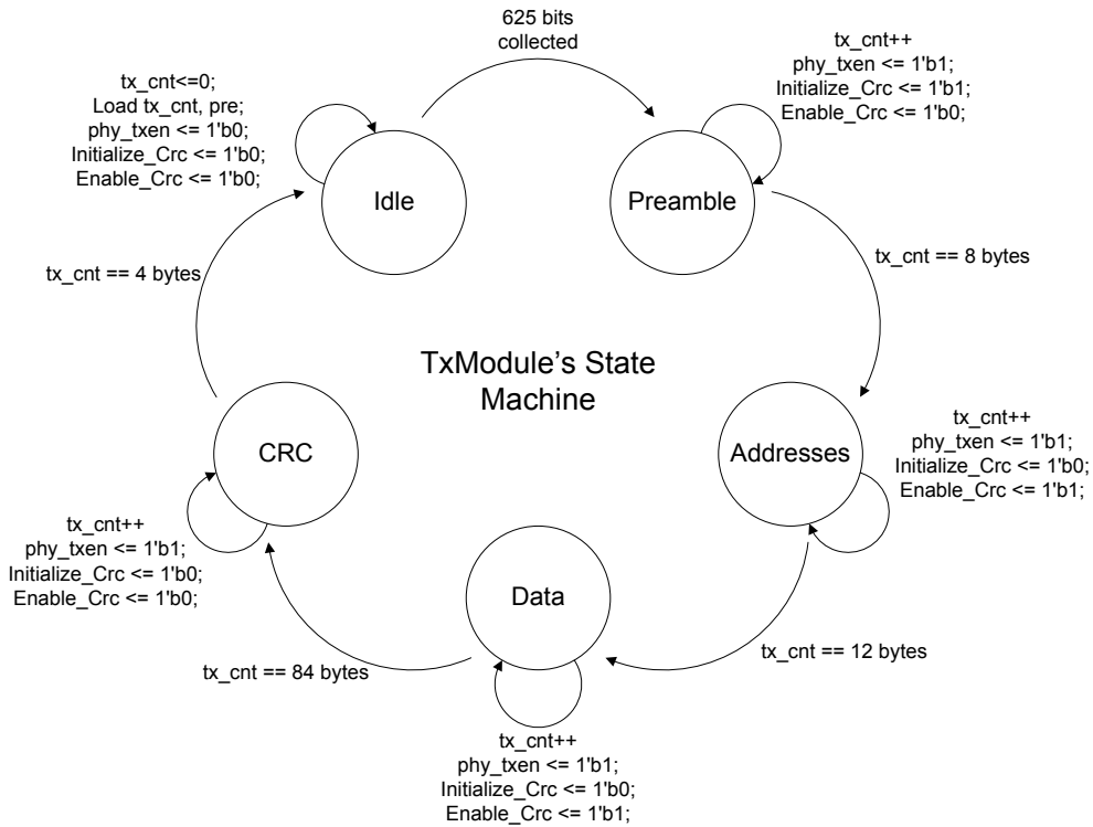
Figure 9 the State Machine of TxModule
