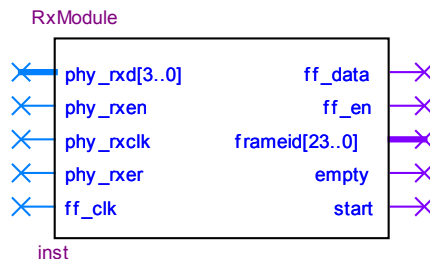
Figure 6 Block Symbol of RxModule
