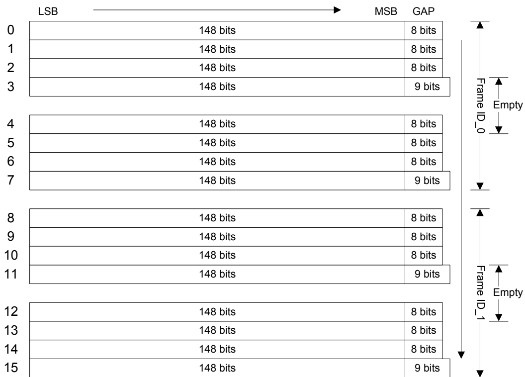
Figure 7 Internal Register Structure & How it works
