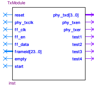
Figure 8 Block Symbol of TxModule
