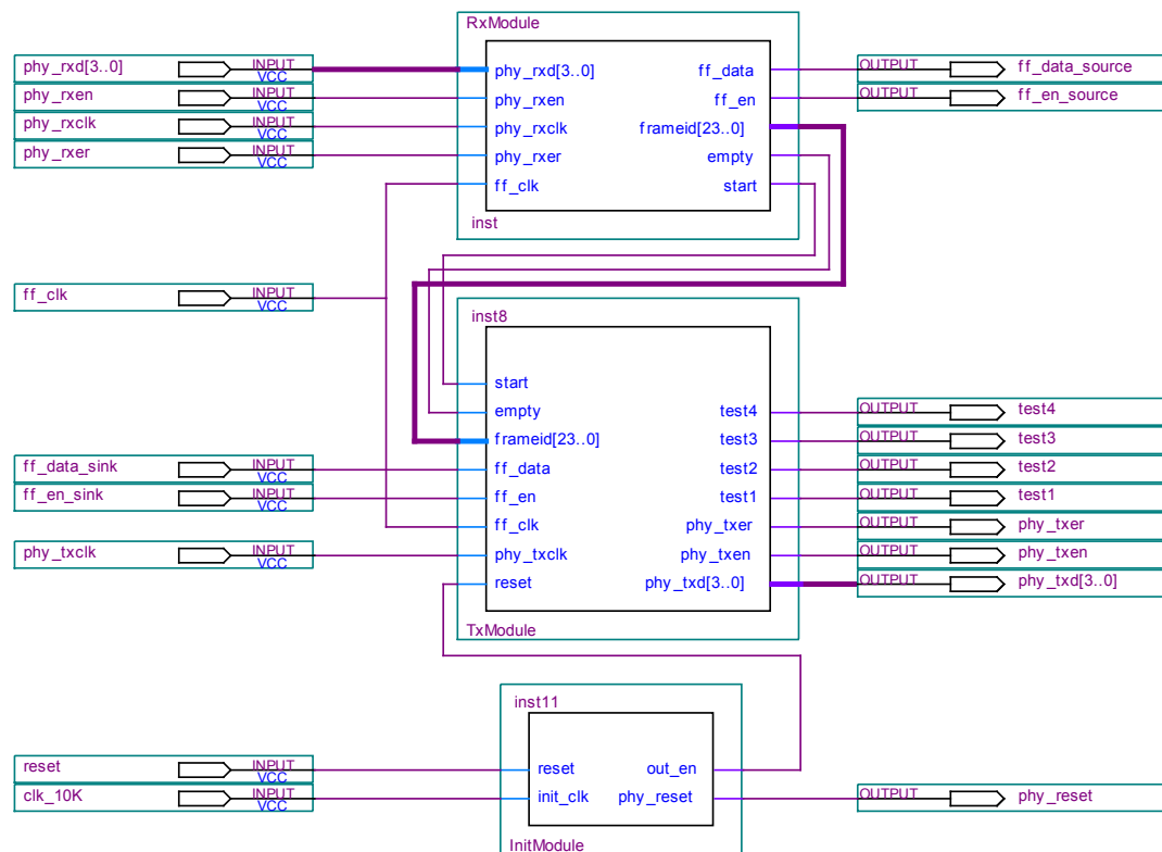
Figure 3 the Top Level Architecture
