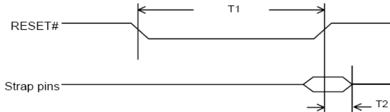
Figure 5 Waveform Shown the Timing Requirement to Reset DM9161
