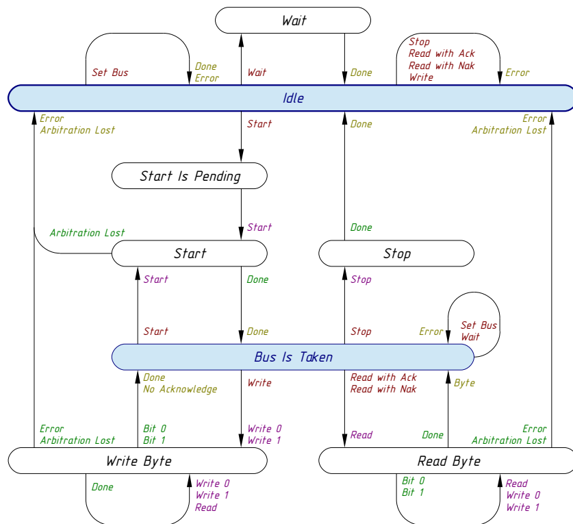
Figure 3: Byte-level FSM
