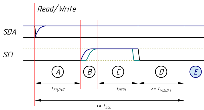
Figure 7: Read/Write waveform
