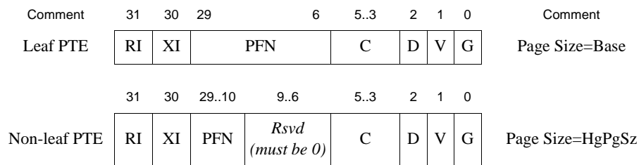
Figure 4.15 8-Byte Rotated PTE Formats
