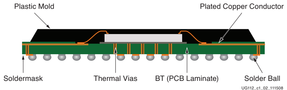
Figure 1-2: Cavity-Up Ball Grid Array Package
