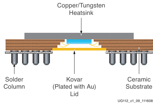
Figure 1-9: CG560 Package
