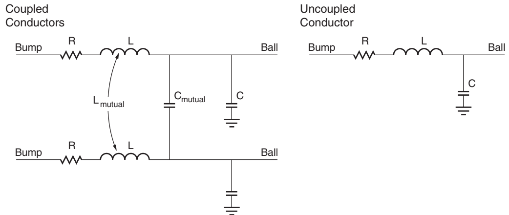
Figure 4-6: Topology of Extracted RLC Parasitic
