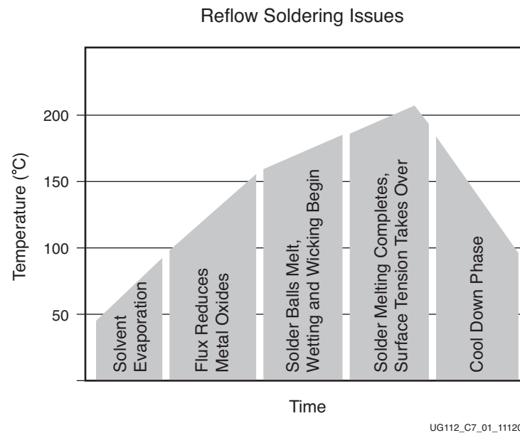
Figure 7-1: Soldering Sequence
