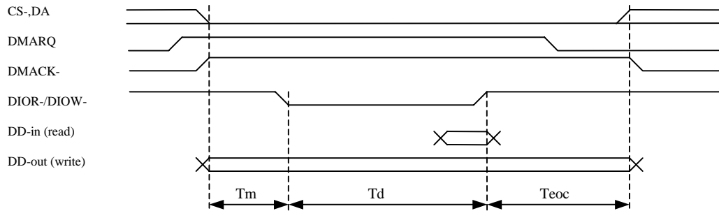
Figure 4.6 DMA Transfer Cycle, terminated by device
