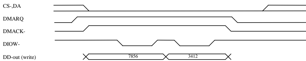
Figure 4.8 32bit DMA write transfer, with endian conversion
