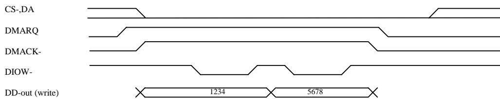
Figure 4.7 32bit DMA write transfer, without endian conversion
