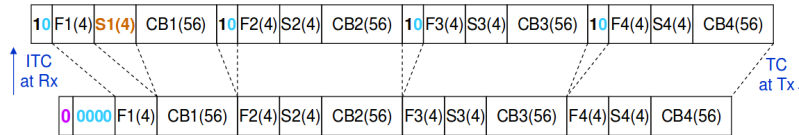
Figure 8: The header of a 256b/257b transmission containing data.
