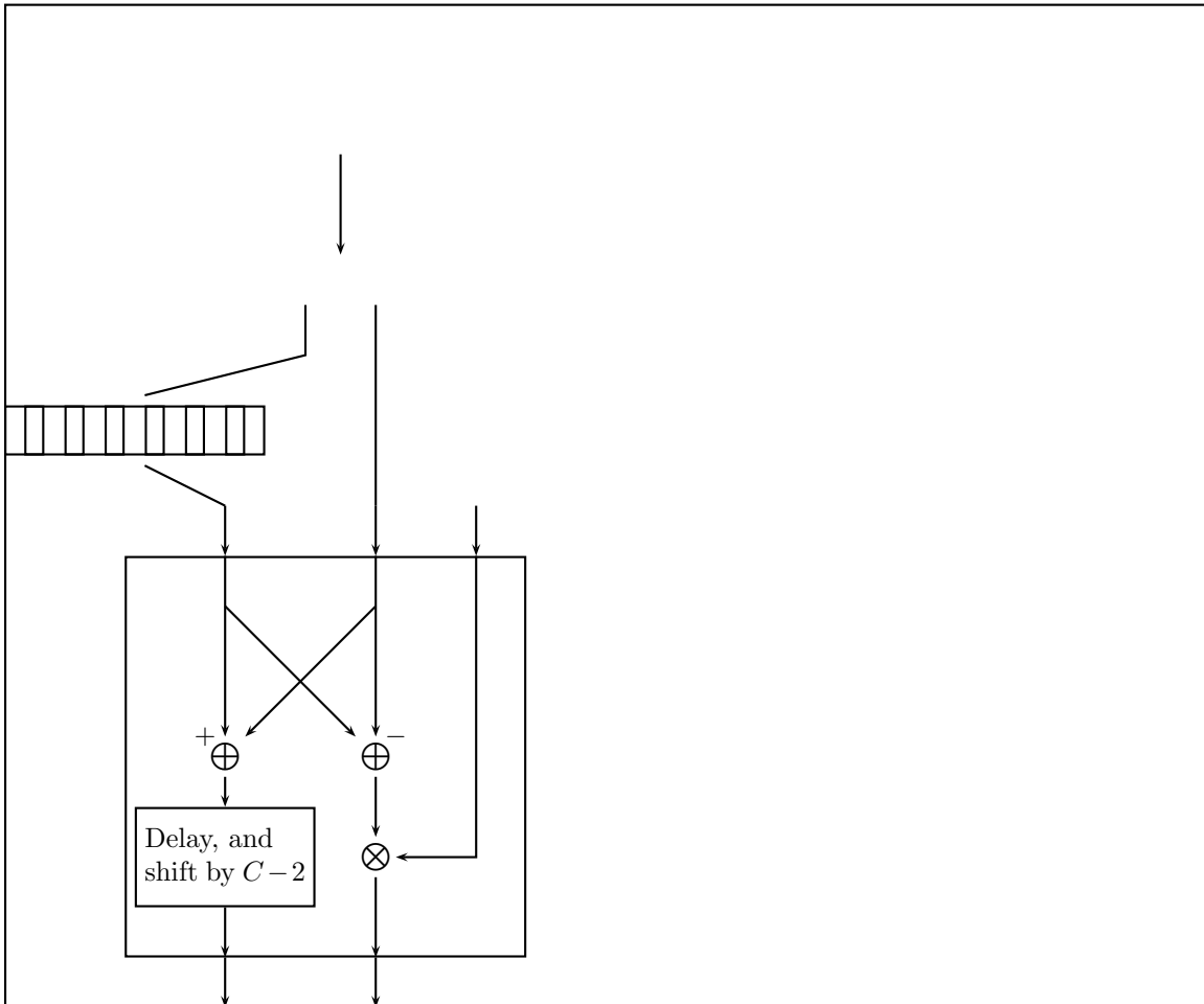
Figure 3.3: A Single FFT Stage, with Butterfly (Figure is still a work in progress)
