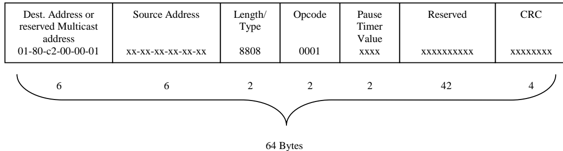
Figure 4: Structure of the PAUSE control frame
