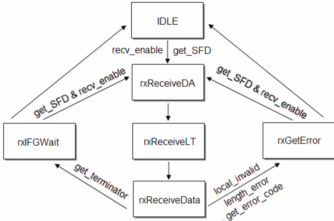
Figure 2-8 block diagram of rxStateMachine
