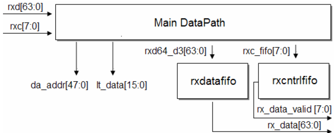
Figure 2-7 block diagram of rxDataPath
