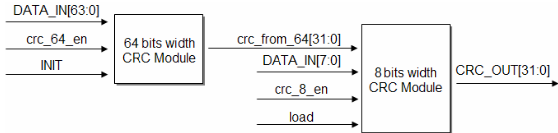
Figure 2-6 block diagram of rxCRCChecker
