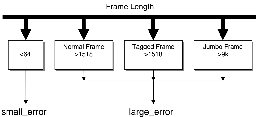
Figure 2-4 block diagram of rxLenTypChecker
