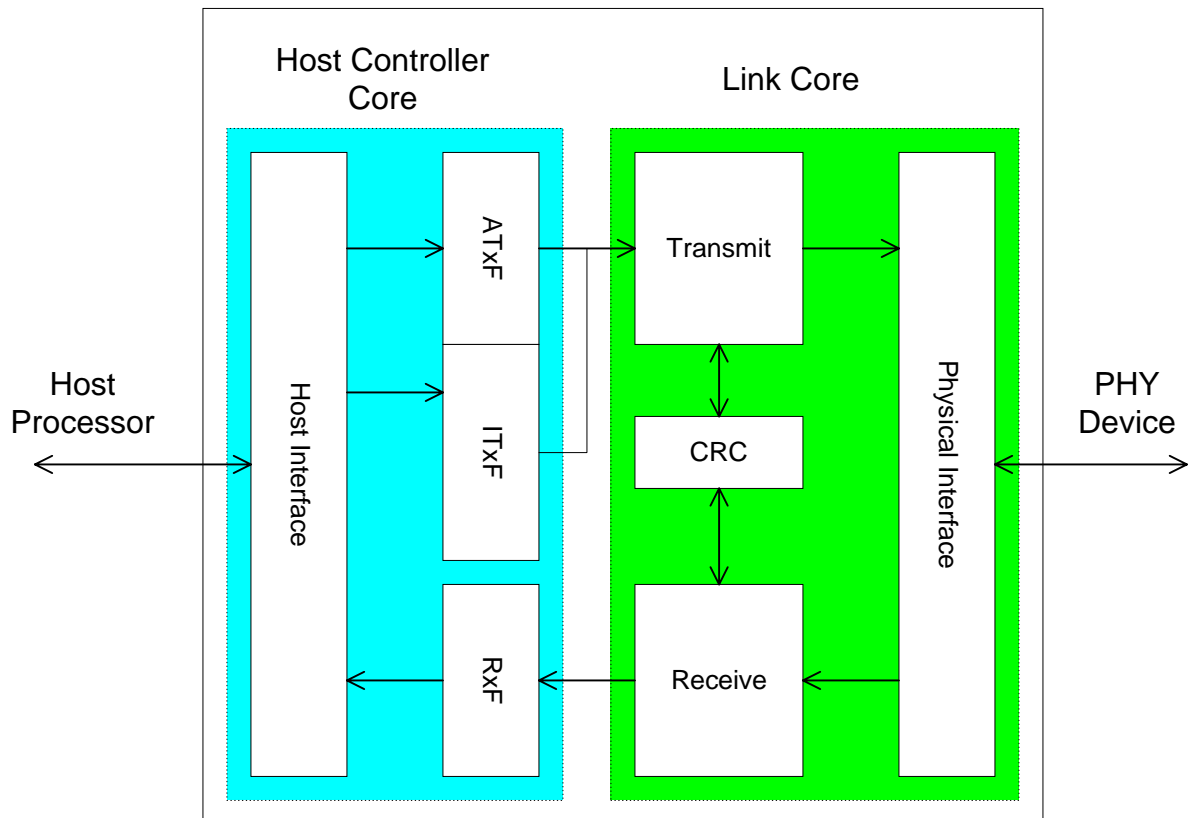
Figure 2.1 Link Layer Cores Block Diagram
