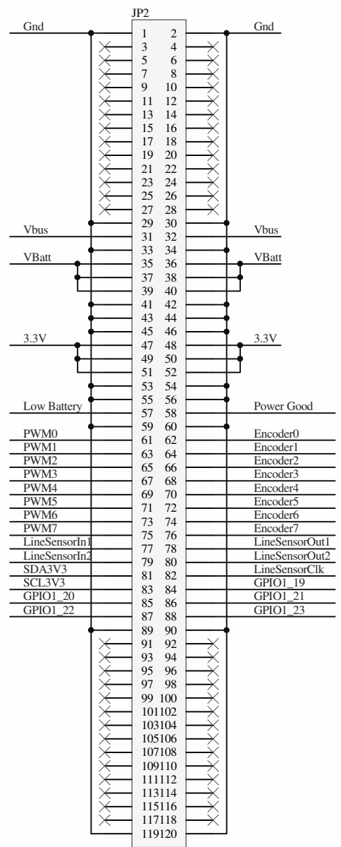
AMP-FH-120-RECEPTABLE-H5
