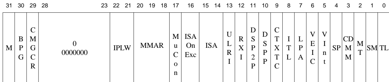
Figure 9-31 Config3 Register Format
