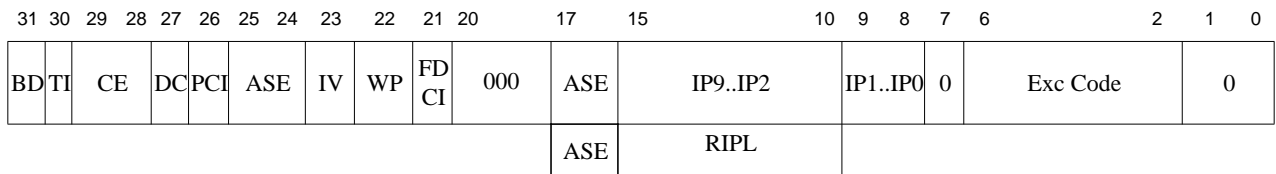
Figure 9-23 Cause Register Format
