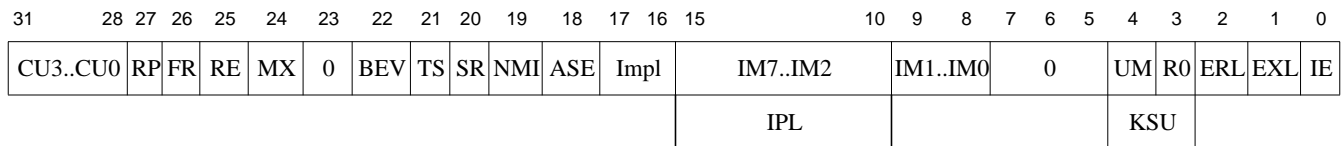
Figure 9-19 Status Register Format
