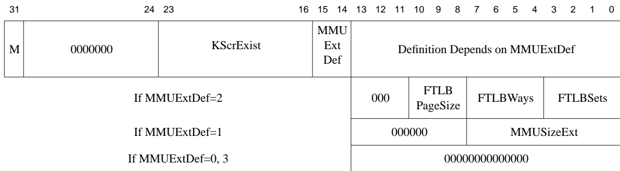
Figure 9-32 Config4 Register Format
