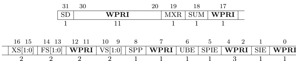
Figure 8.21: Virtual supervisor status register ( vsstatus ) when VSXLEN=32.
