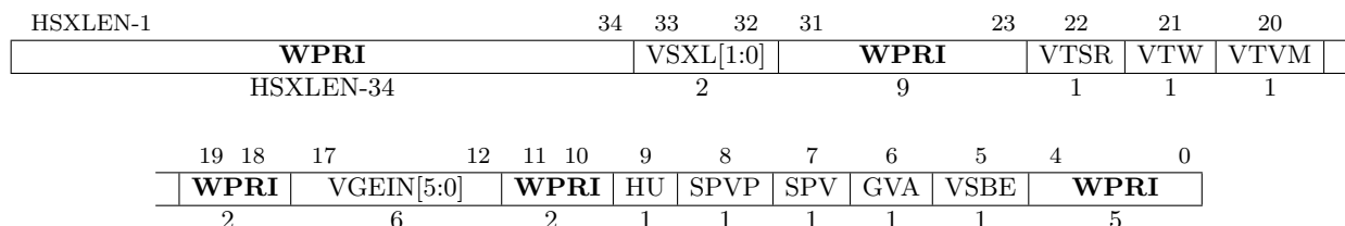
Figure 5.2: Hypervisor status register ( hstatus ) when HSXLEN=64.
