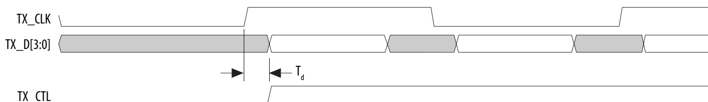
Figure 10: RGMII TX Timing Diagram
