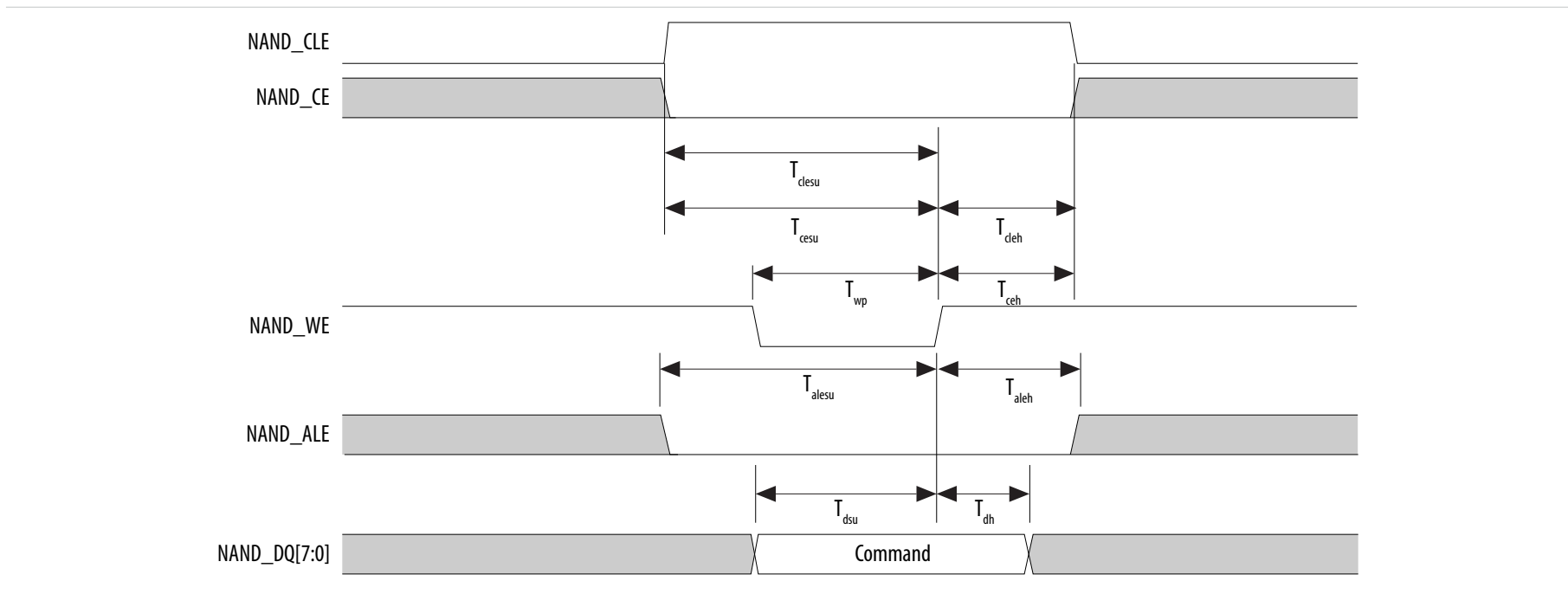
Figure 14: NAND Command Latch Timing Diagram
