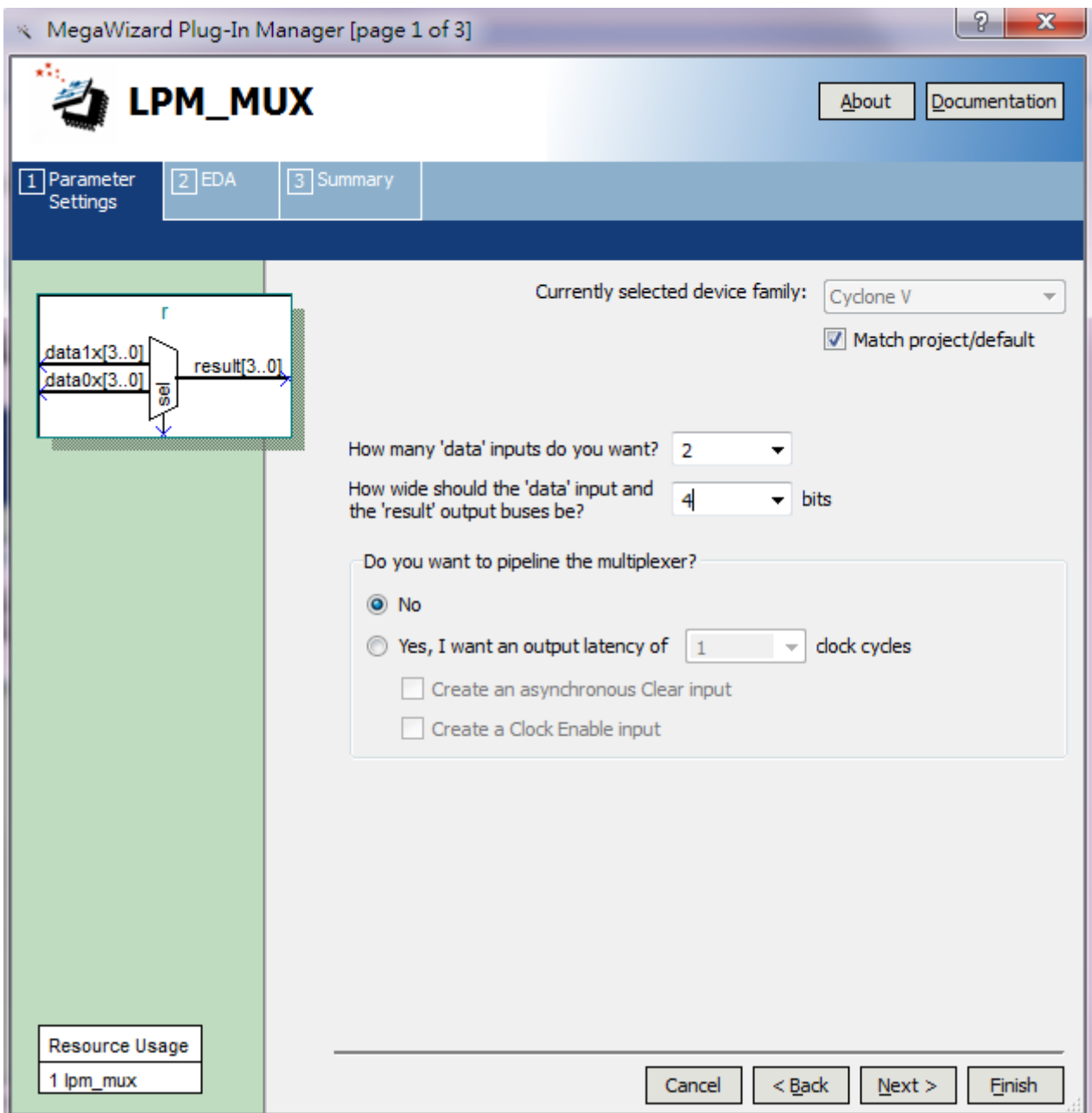
Figure 3-23 lpm_mux settings
