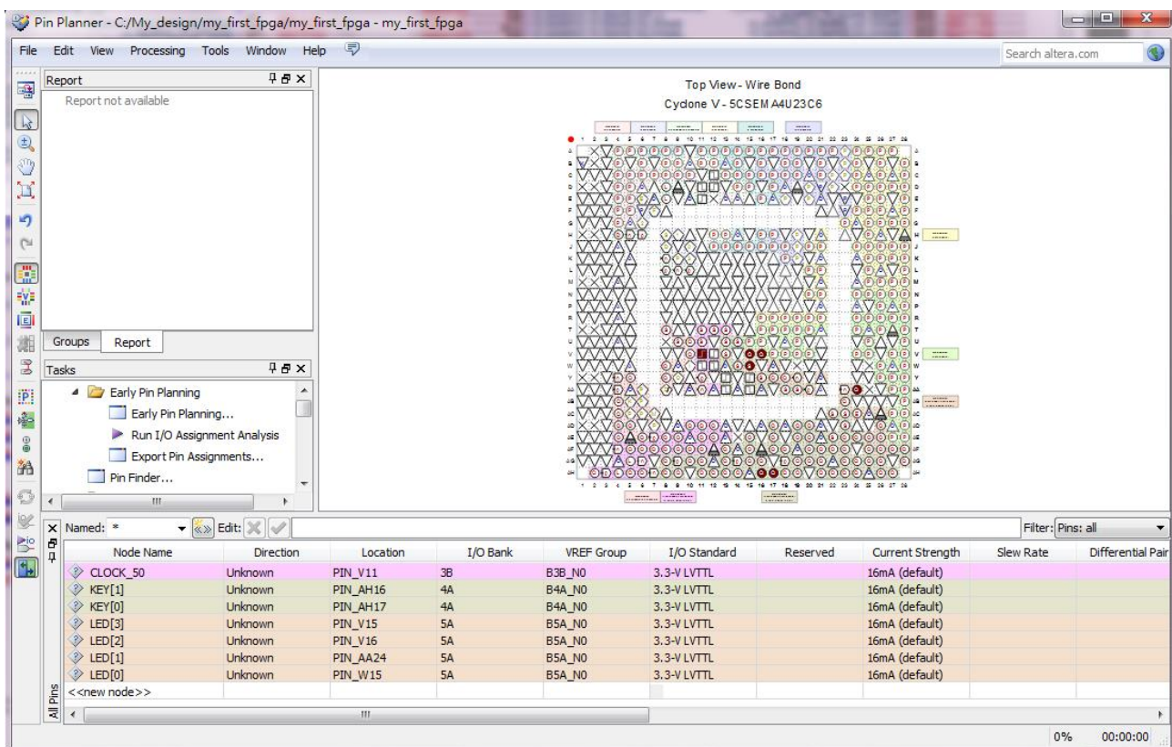
Figure 3-33 Completed Pin Planning Example
