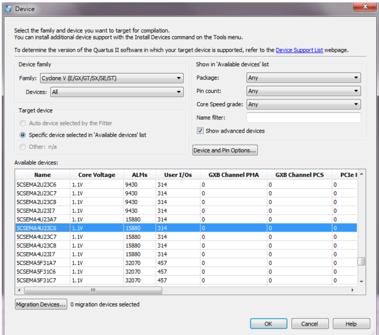
Figure 2-3 Specify the Device Example
