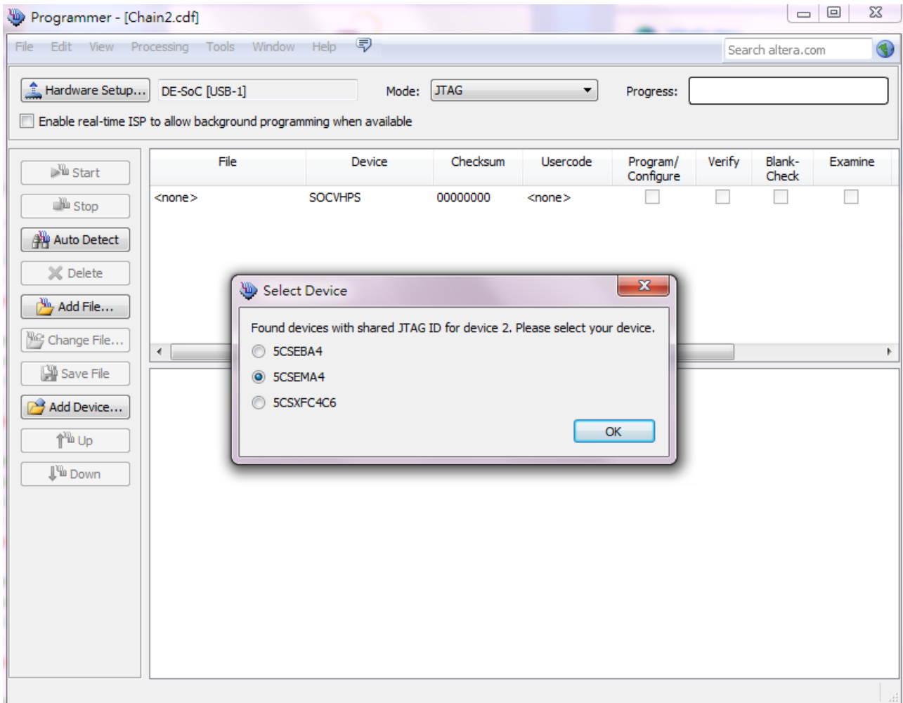
Figure 4-5 Select FPGA Device
