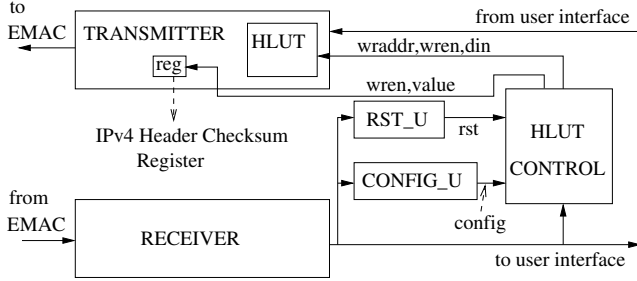
Figure 1. Top-level design of the advanced UDP/IP core.
