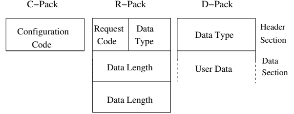
Figure 2. Supported packets in the Configuration and Data Protocol.
