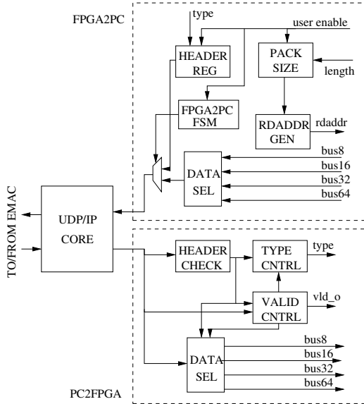
Figure 3. Hardware design of the communication platform.
