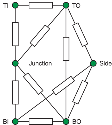
Figure 3-6: Compact Thermal Model Topologies
