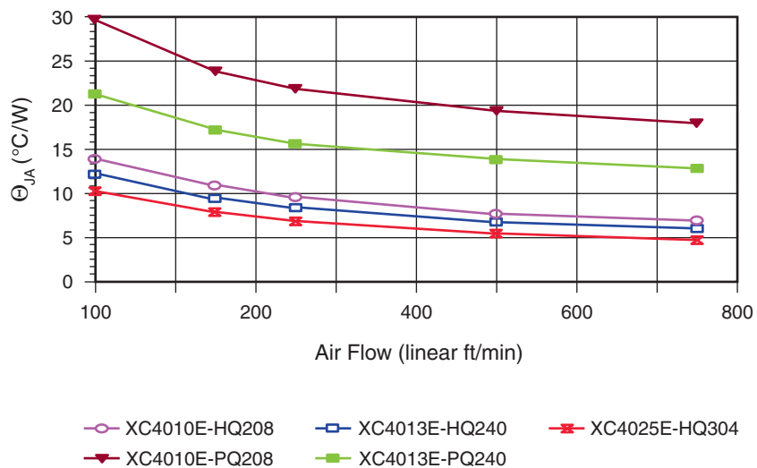
Figure 3-8: Effect of Air Flow on the Thermal Resistance ( \theta_{JA} ) of HQ/PQ Packages
