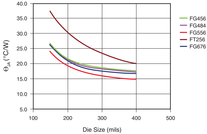
Figure 3-7: Effect of Die Size on the Thermal Resistance ( \theta_{JA} ) of PBGA Packages
