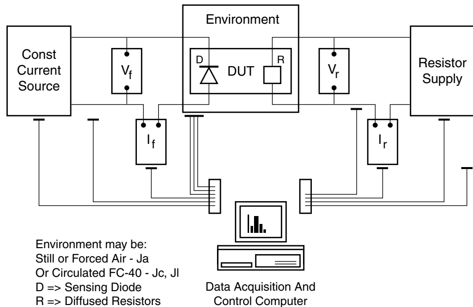
Figure 3-2: Thermal Measurement Setup (Schematic for Junction to Reference)
