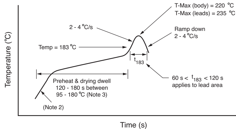
Figure 7-3: Typical Conditions for IR Reflow Soldering of Sn/Pb Solder
