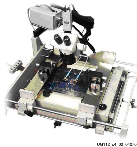
Figure 4-2: GTL VNA Fixture
