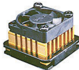
Figure 3-14: Example of Active Heatsink for BGA (Malico)
