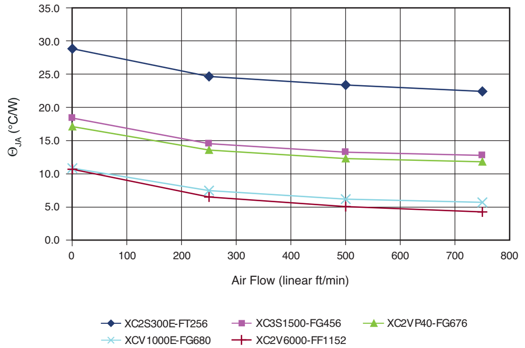
Figure 3-10: Effect of Air Flow on the Thermal Resistance ( \theta_{JA} ) of BGA Packages
