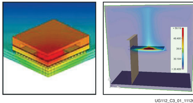
Figure 3-1: Simulation Tool Outputs: a) Quarter Model of a Package, b) CTM in JEDEC Enclosure
