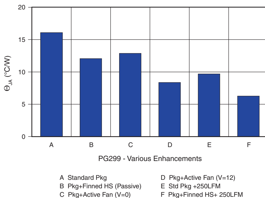
Figure 3-9: Effect of Active and Passive Heat Sinks on the Thermal Resistance ( \theta_{JA} ) of PG299 Packages
