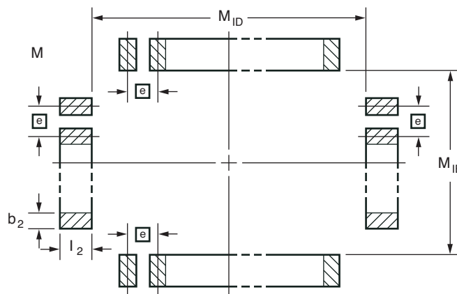
Figure 5-1: EIA Standard Board Layout of Soldered Pads for QFP Packages
