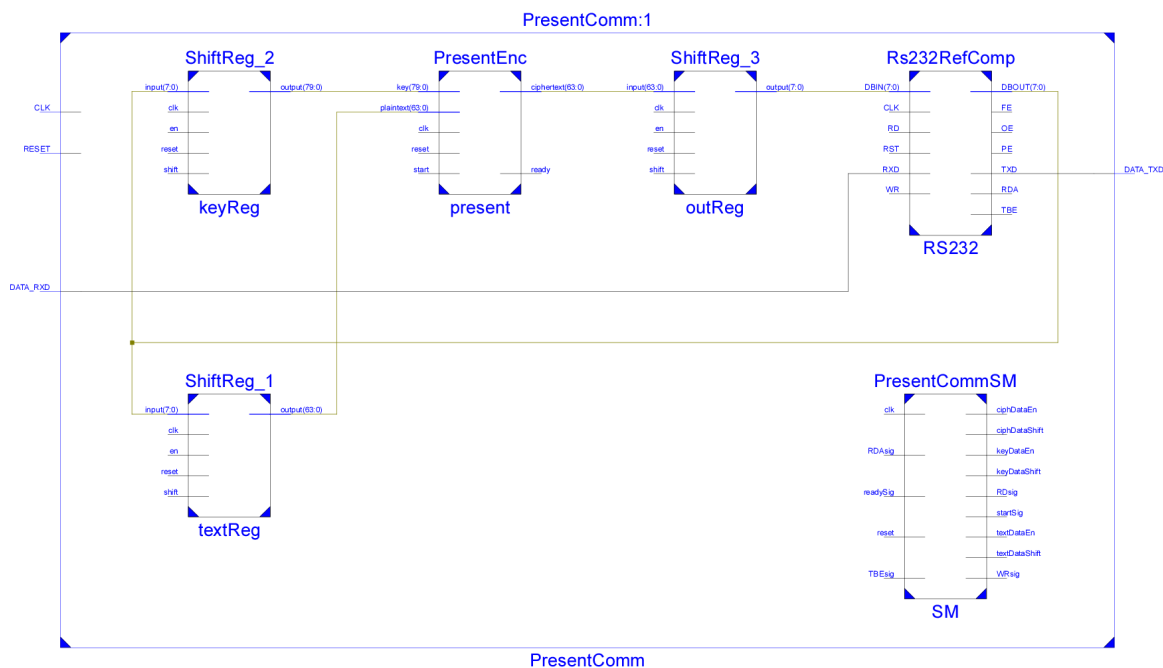
Figure 3: Internal structure of Present core with communication environment.
