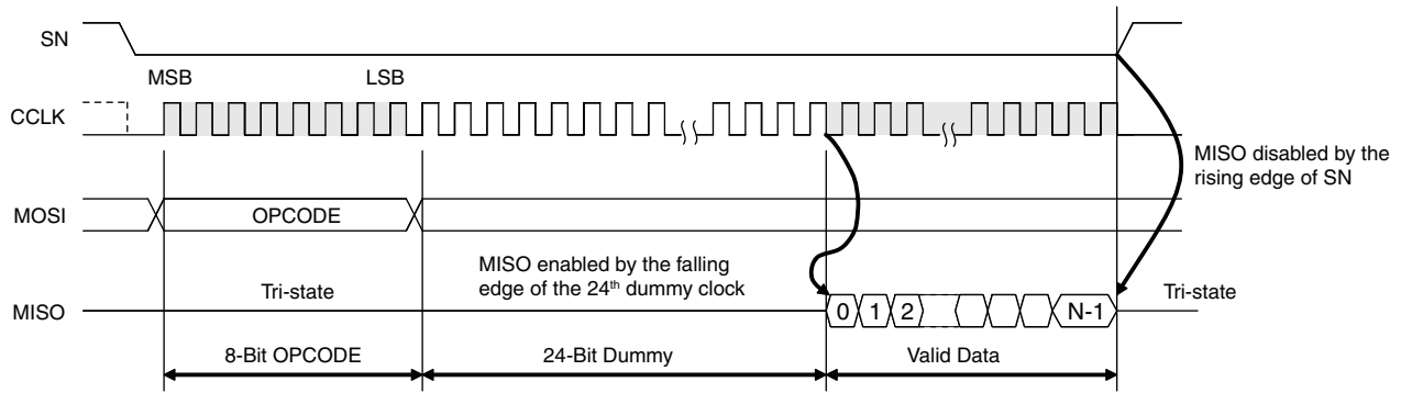
Figure 16. Class A Command Waveforms
