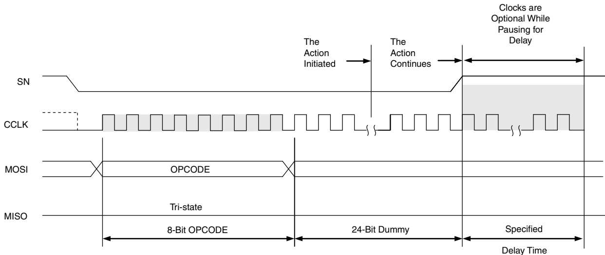
Figure 19. Class D Command Waveforms
