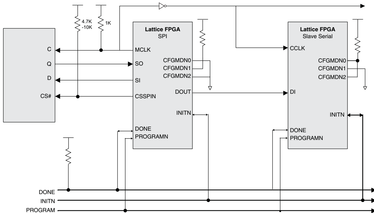
Figure 26. Serial Daisy Chaining
