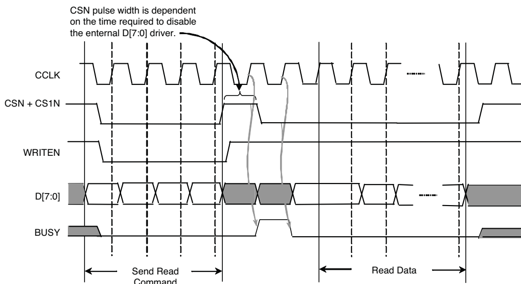
Figure 22. Slave Parallel Read
