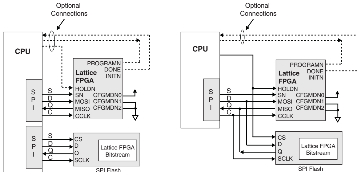
Figure 11. ECP5 and ECP5-5G Slave SPI Port with SPI Flash
