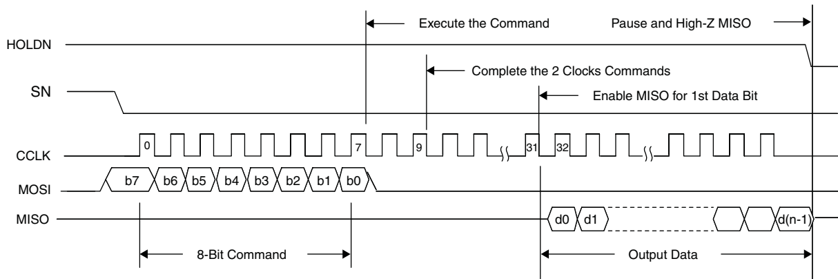
Figure 12. Slave SPI Read Waveforms
