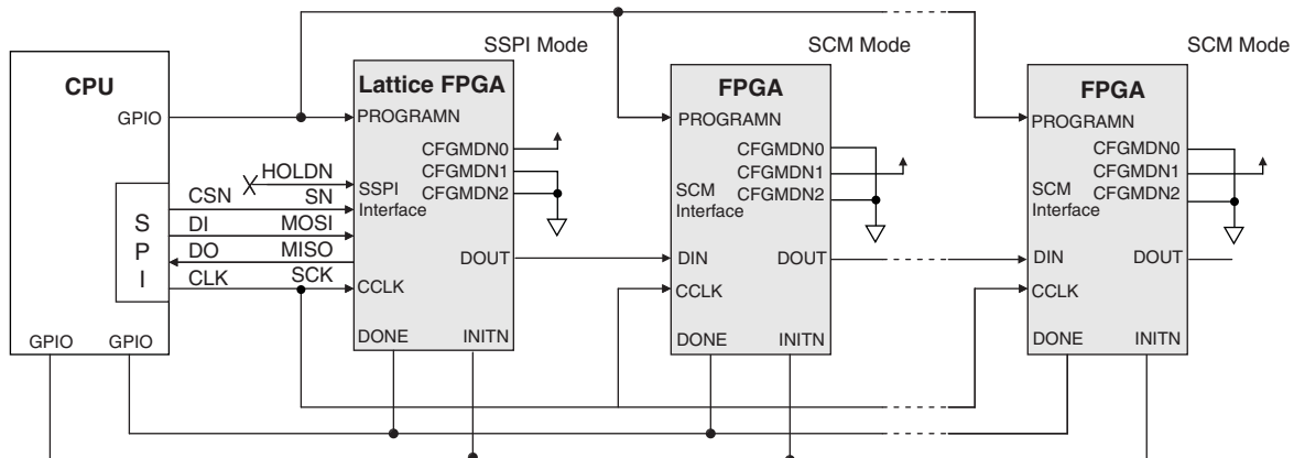
Figure 31. Slave SPI sysCONFIG Daisy Chain
