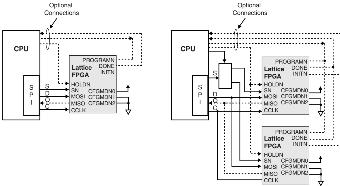
Figure 10. ECP5 and ECP5-5G Slave SPI Port with CPU and Single or Multiple Devices
