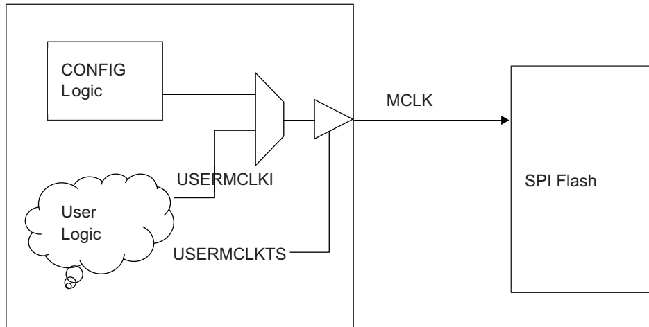
Figure 7. MCLK Connection
