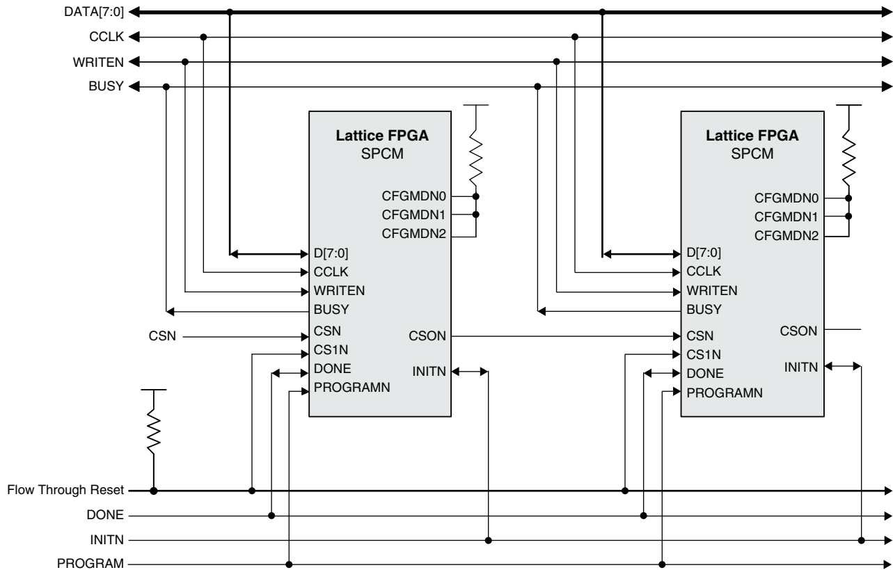
Figure 28. SPCM Configuration with Daisy Chaining
