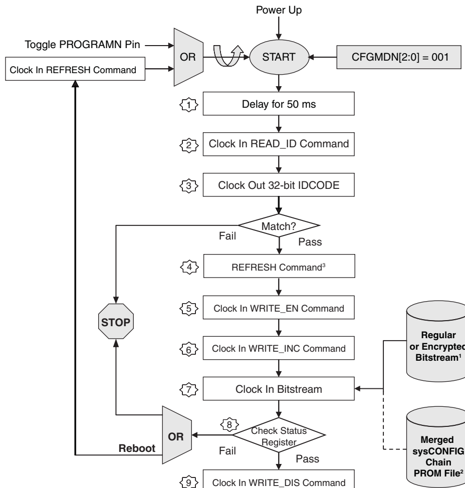
Figure 15. Slave SPI Configuration Flow Diagram
