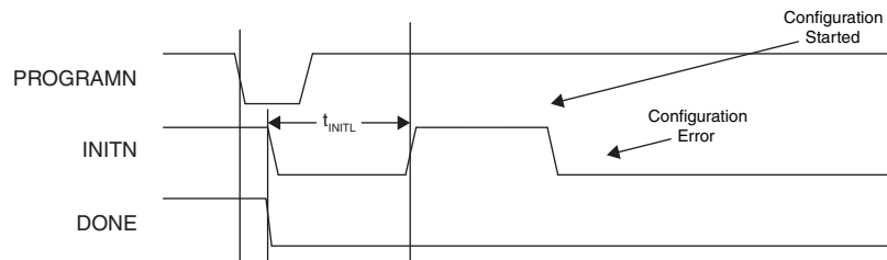
Figure 2. Configuration Error Notification
