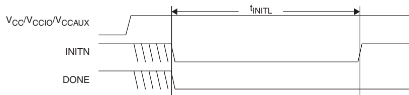
Figure 5. Configuration from Power-On-Reset Timing
