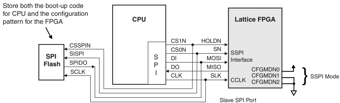
Figure 29. Example Slave SPI System Diagram (Slave SPI Mode)
