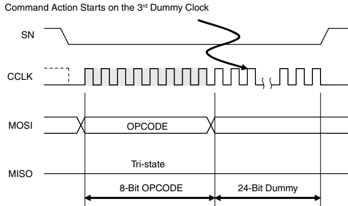
Figure 18. Class C Command Waveforms
