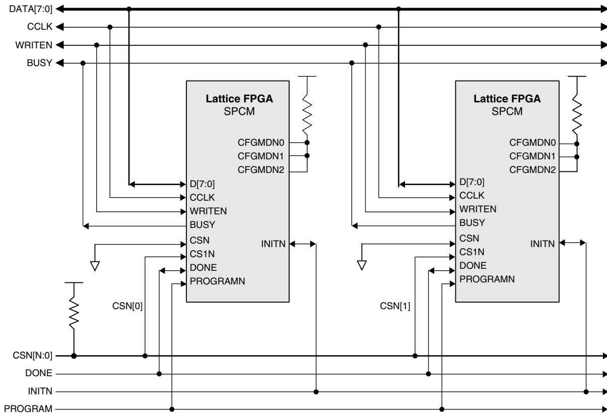
Figure 20. Slave Parallel Interface
