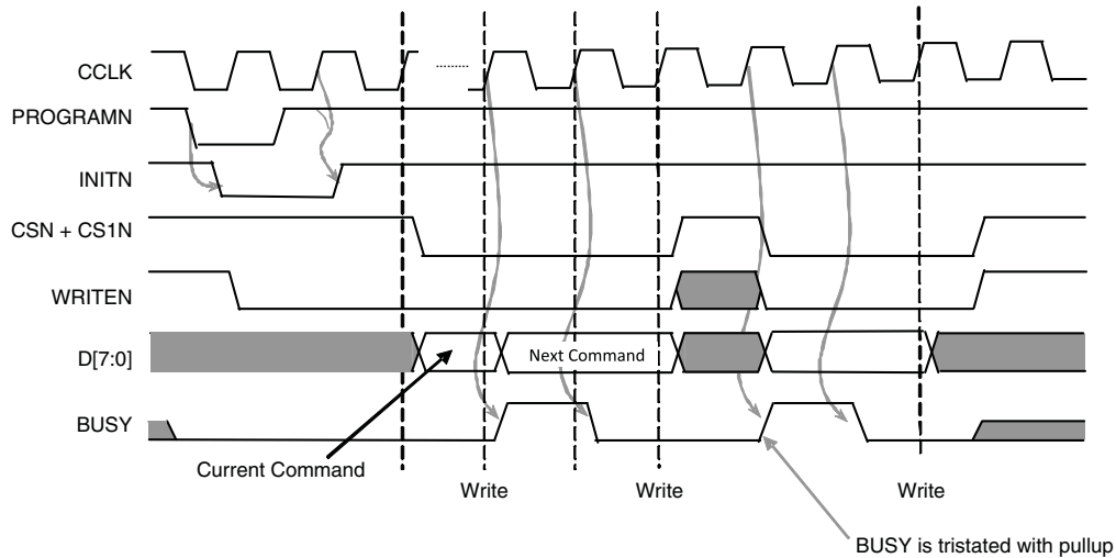
Figure 21. Slave Parallel Write
