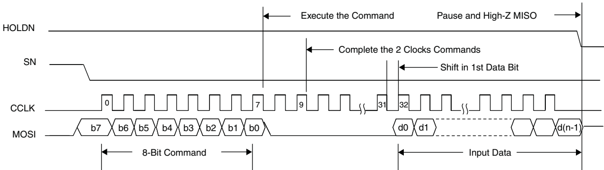
Figure 13. Slave SPI Write Waveforms
