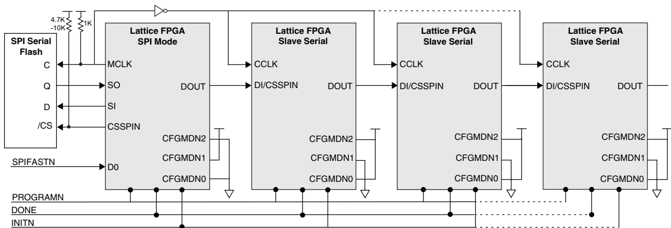
Figure 30. Master SPI sysCONFIG Daisy Chain
