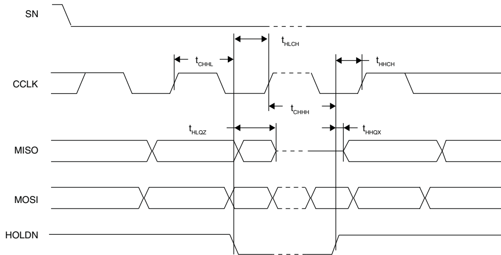
Figure 14. Slave SPI HOLDN Waveforms
