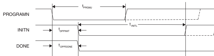
Figure 1. Configuration from PROGRAMN Timing
