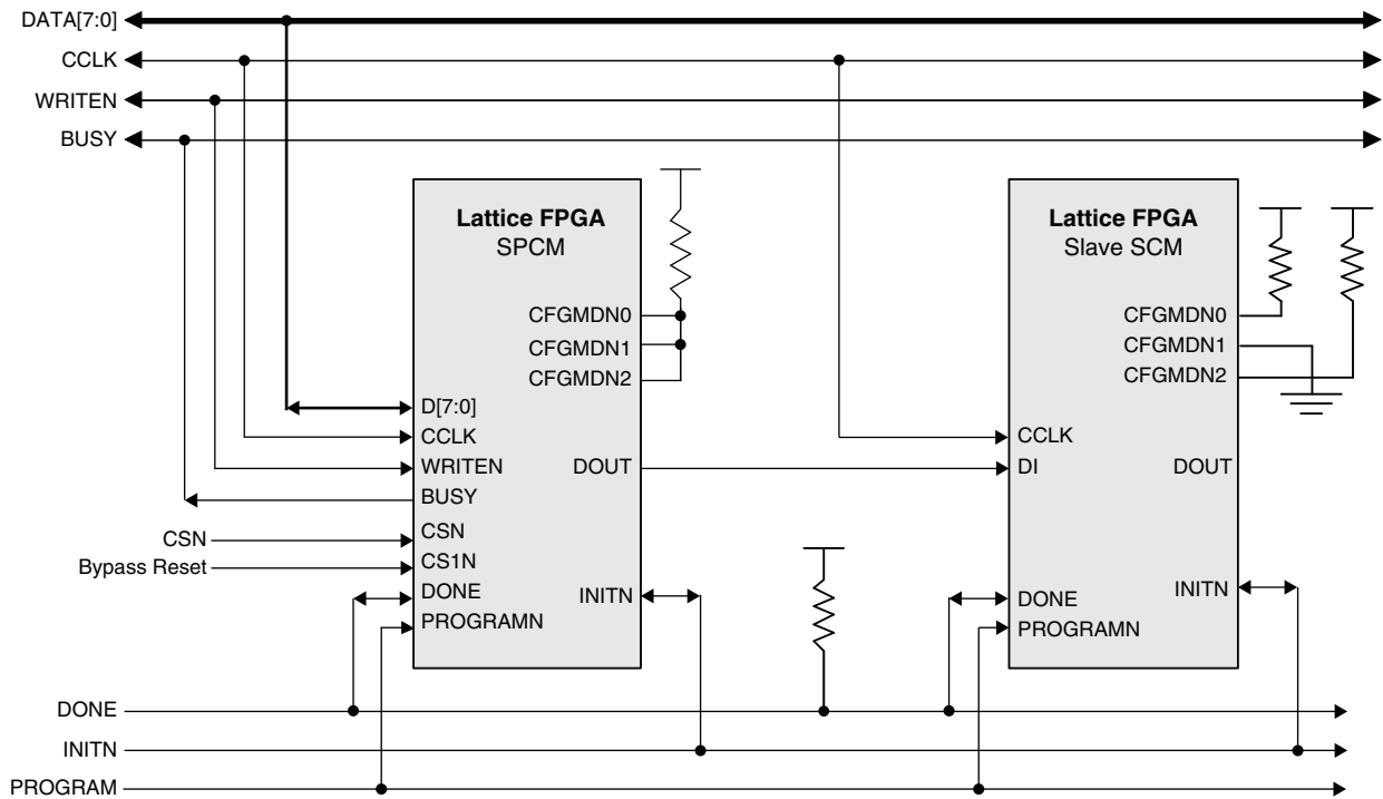
Figure 27. SPCM with Serial Daisy Chain
