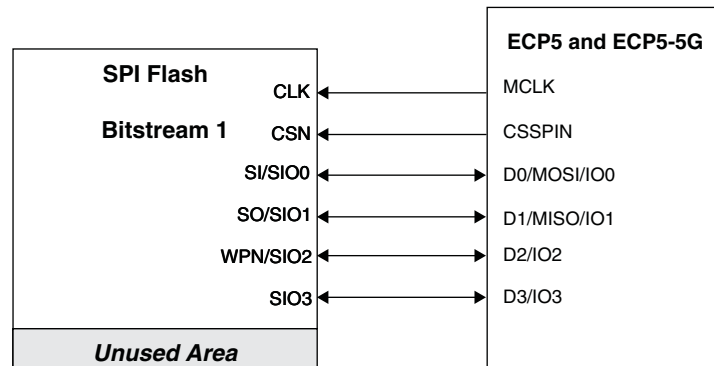
Figure 9. One Quad SPI Flash Interface (Quad)
