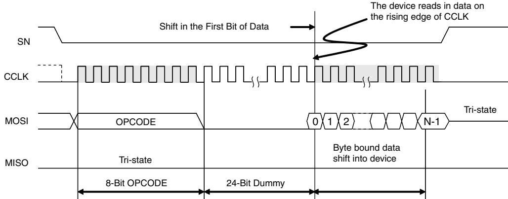
Figure 17. Class B Command Waveforms
