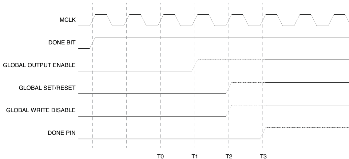
Figure 25. Wake-up Sequence Using Internal Clock
