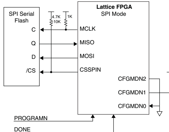
Figure 6. ECP5 and ECP5-5G Master SPI Port with SPI Flash
