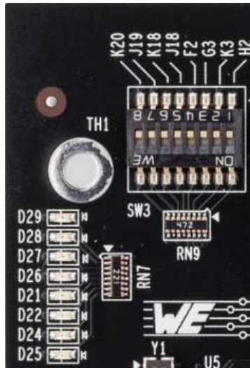
Figure 11. ECP5-5G Versa Development Board LEDs and Switches
