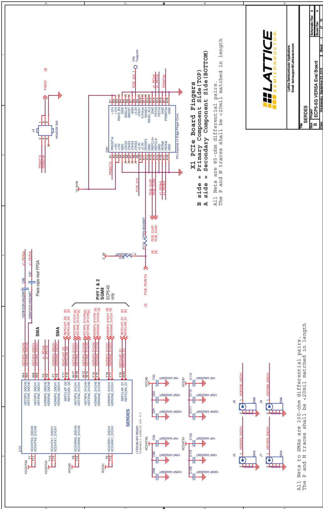
Figure 16. SERDES
