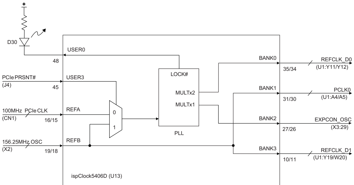
Figure 9. Clock Controller Scheme
