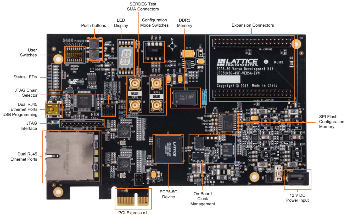
Figure 1. ECP5-5G Versa Development Board, Top Side
