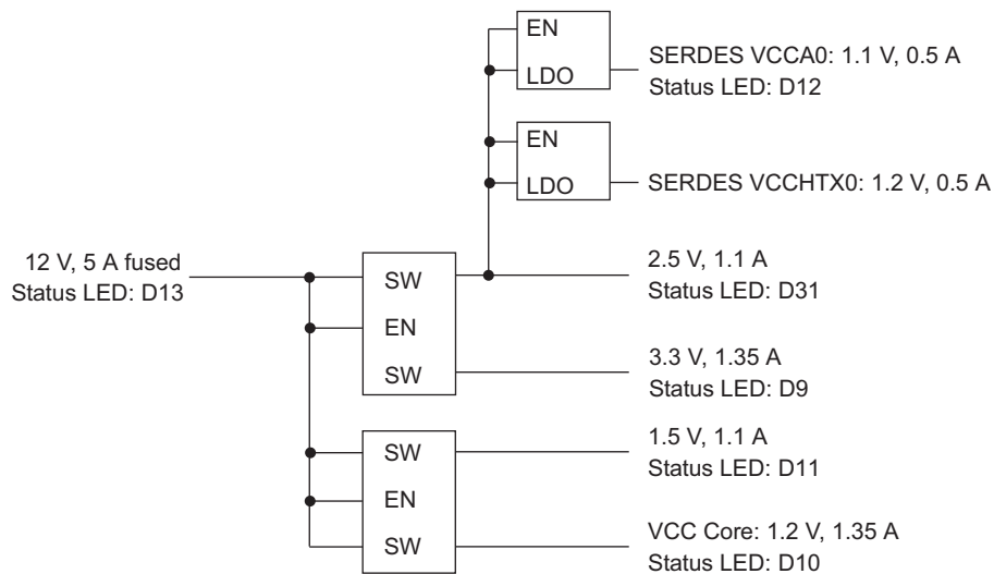
Figure 2. Power Distribution Scheme (See Appendix A, Sheet 2, Figure 14- Voltage Regulators)
