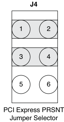
Figure 10. PCI Express PRSNT Control Connection
