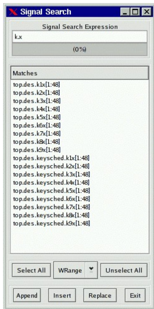
Figure 16: The Signal Search (regular expression search) Requester
