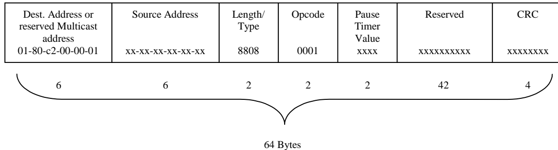
Figure 1: Structure of the PAUSE control frame
